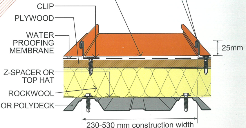
S25 YODO STANDING SEAM
